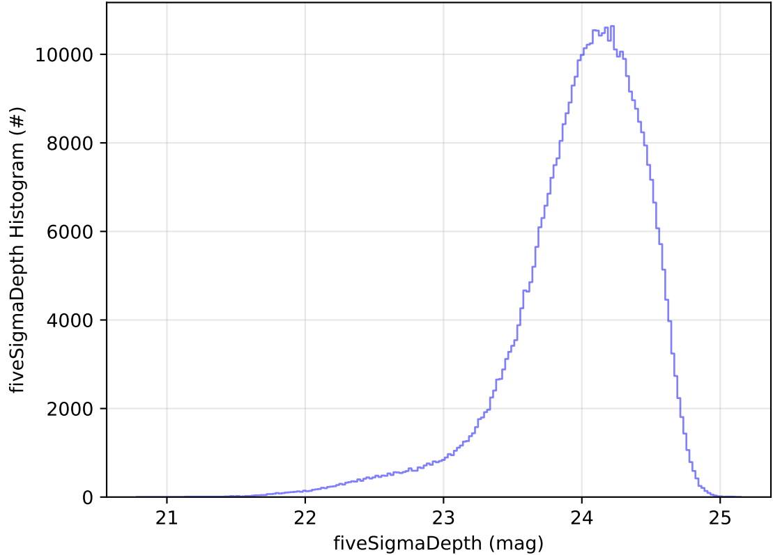
ddf_acor_sf25_lsf40_lsr10_v3.4_10yrs WFD r band: fiveSigmaDepth Histogram
