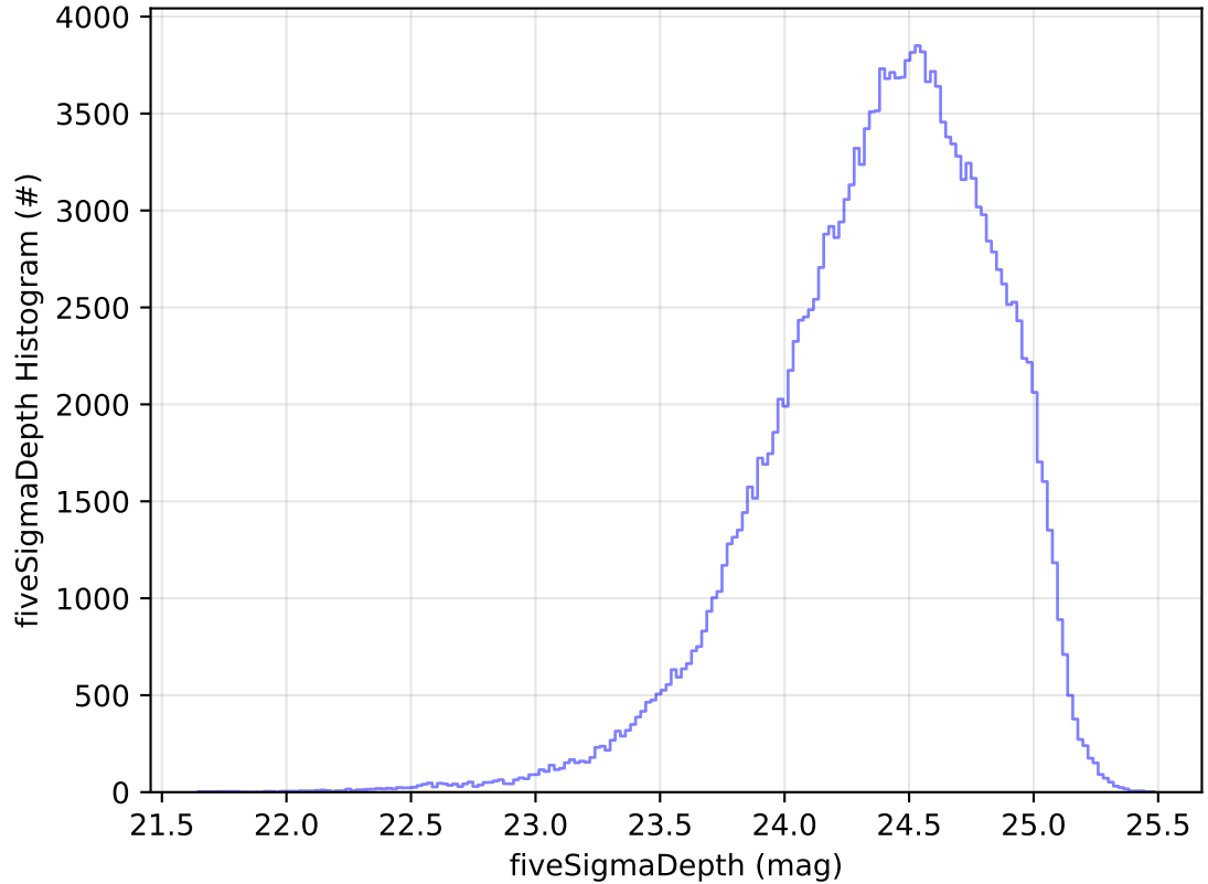
ddf_acor_sf25_lsf40_lsr10_v3.4_10yrs WFD g band: fiveSigmaDepth Histogram
