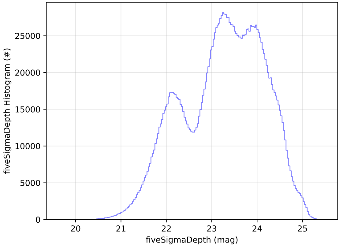
ddf_acor_sf25_lsf40_lsr10_v3.4_10yrs WFD all bands: fiveSigmaDepth Histogram
