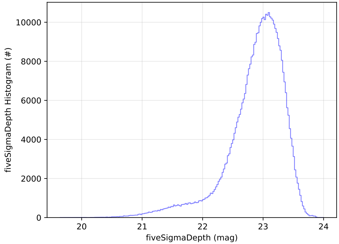
ddf_acor_sf25_lsf40_lsr10_v3.4_10yrs All sky z band: fiveSigmaDepth Histogram
