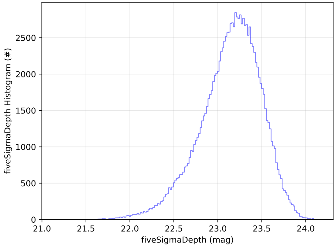
ddf_acor_sf25_lsf40_lsr10_v3.4_10yrs All sky u band: fiveSigmaDepth Histogram
