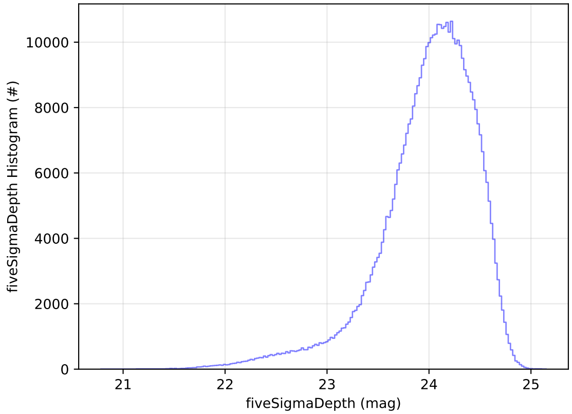
ddf_acor_sf25_lsf40_lsr10_v3.4_10yrs All sky r band: fiveSigmaDepth Histogram
