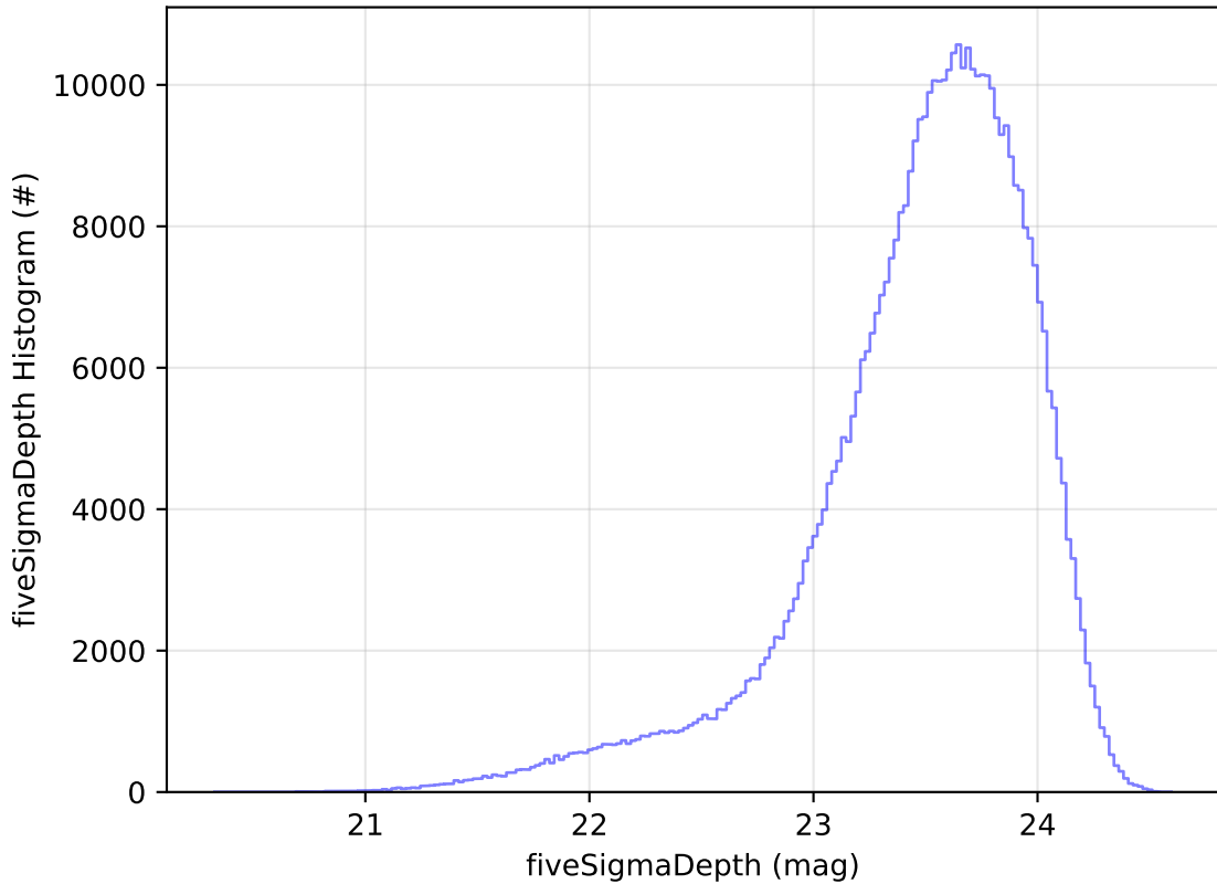
ddf_acor_sf25_lsf40_lsr10_v3.4_10yrs All sky i band: fiveSigmaDepth Histogram
