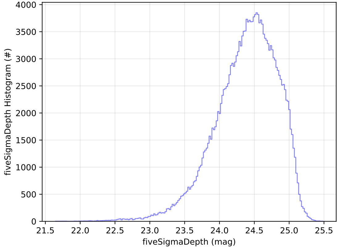
ddf_acor_sf25_lsf40_lsr10_v3.4_10yrs All sky g band: fiveSigmaDepth Histogram
