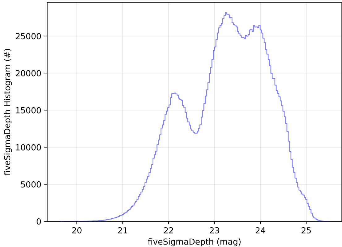
ddf_acor_sf25_lsf40_lsr10_v3.4_10yrs All sky all bands: fiveSigmaDepth Histogram
