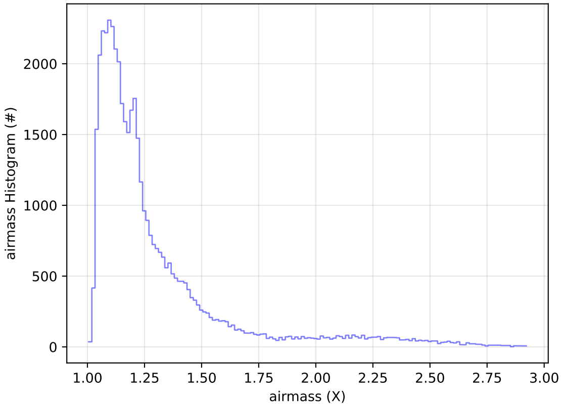
ddf_acor_sf25_lsf40_lsr10_v3.4_10yrs Yr 1 z band: airmass Histogram
