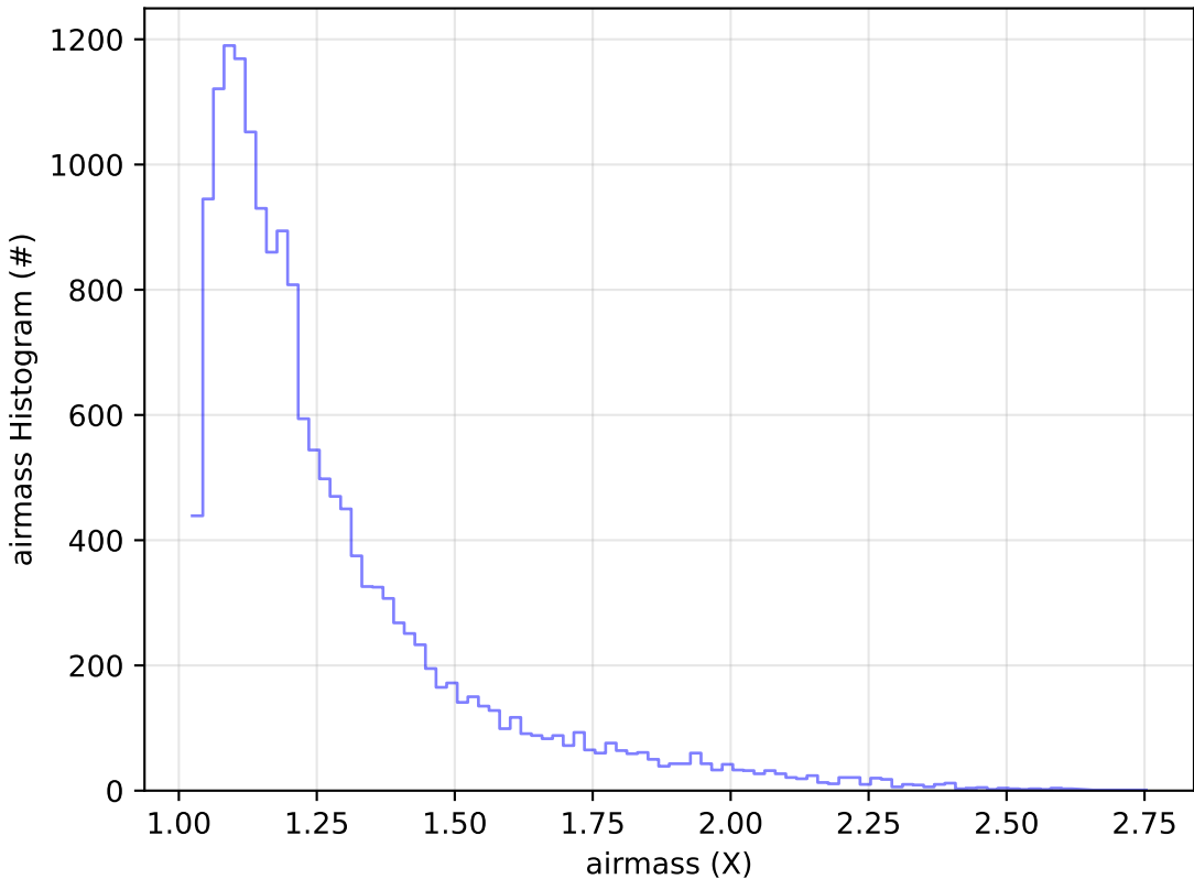
ddf_acor_sf25_lsf40_lsr10_v3.4_10yrs Yr 1 u band: airmass Histogram
