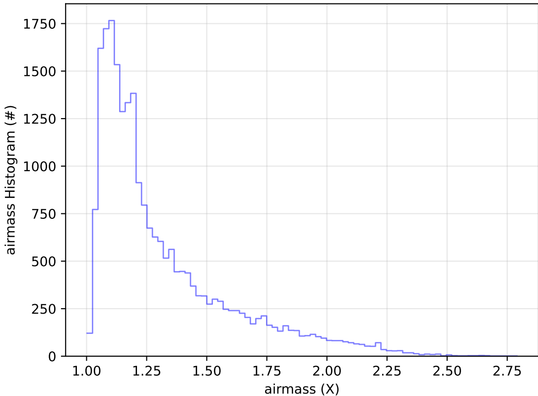
ddf_acor_sf25_lsf40_lsr10_v3.4_10yrs Yr 1 g band: airmass Histogram
