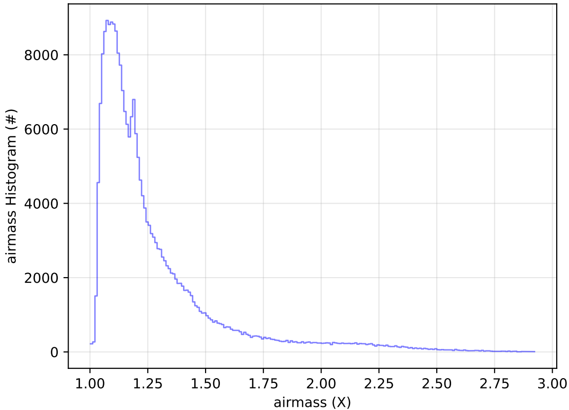
ddf_acor_sf25_lsf40_lsr10_v3.4_10yrs Yr 1 all bands: airmass Histogram
