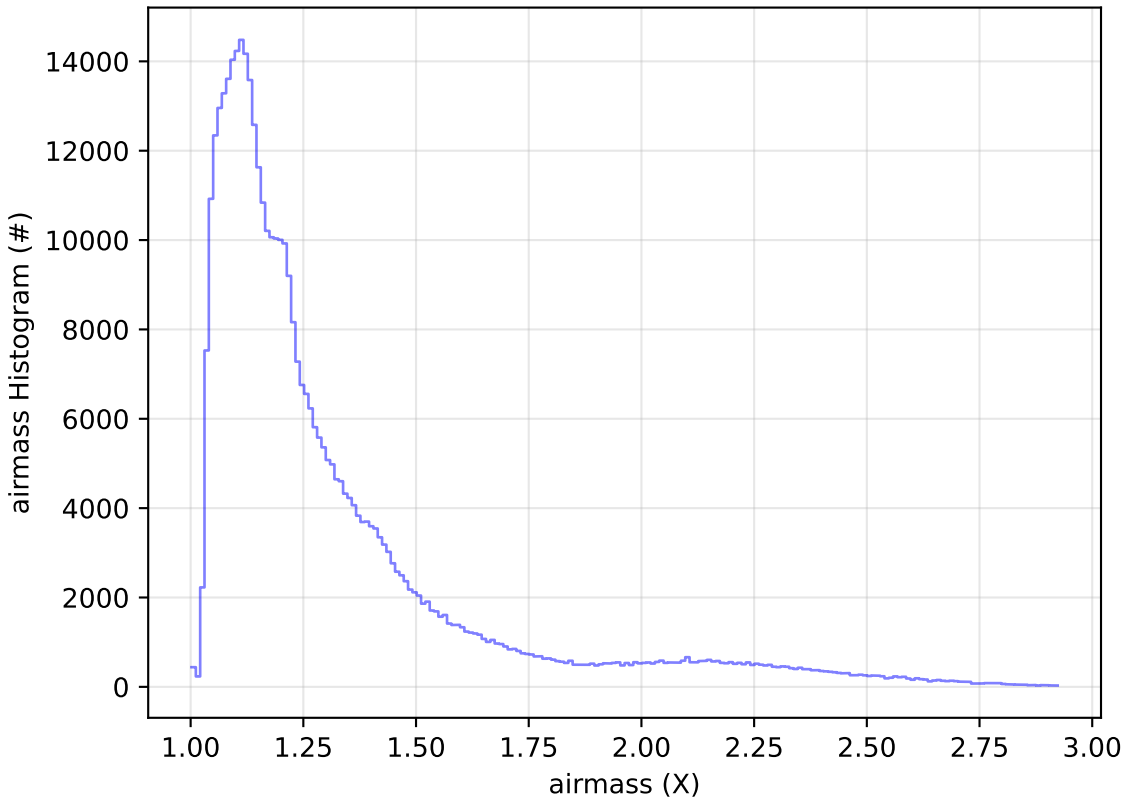
ddf_acor_sf25_lsf40_lsr10_v3.4_10yrs WFD z band: airmass Histogram
