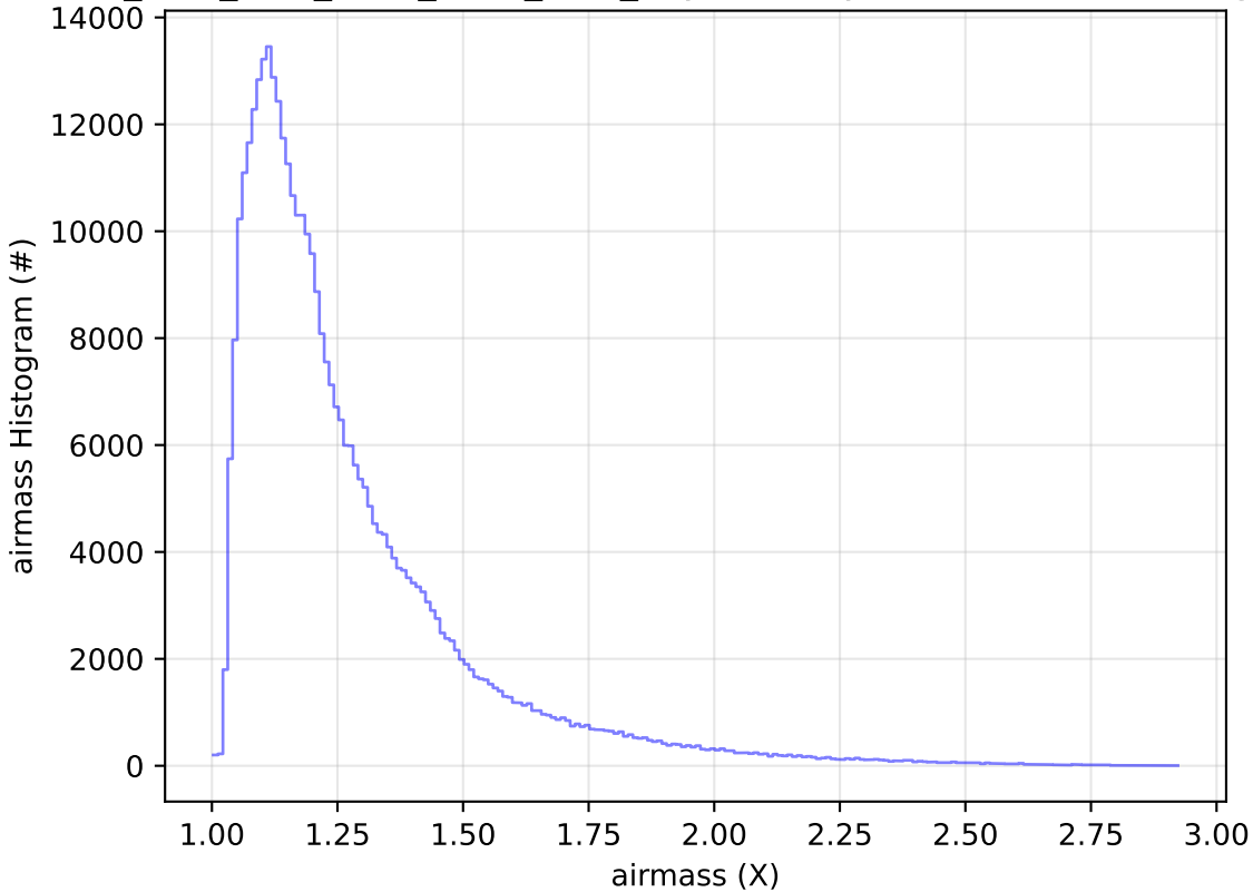
ddf_acor_sf25_lsf40_lsr10_v3.4_10yrs WFD y band: airmass Histogram
