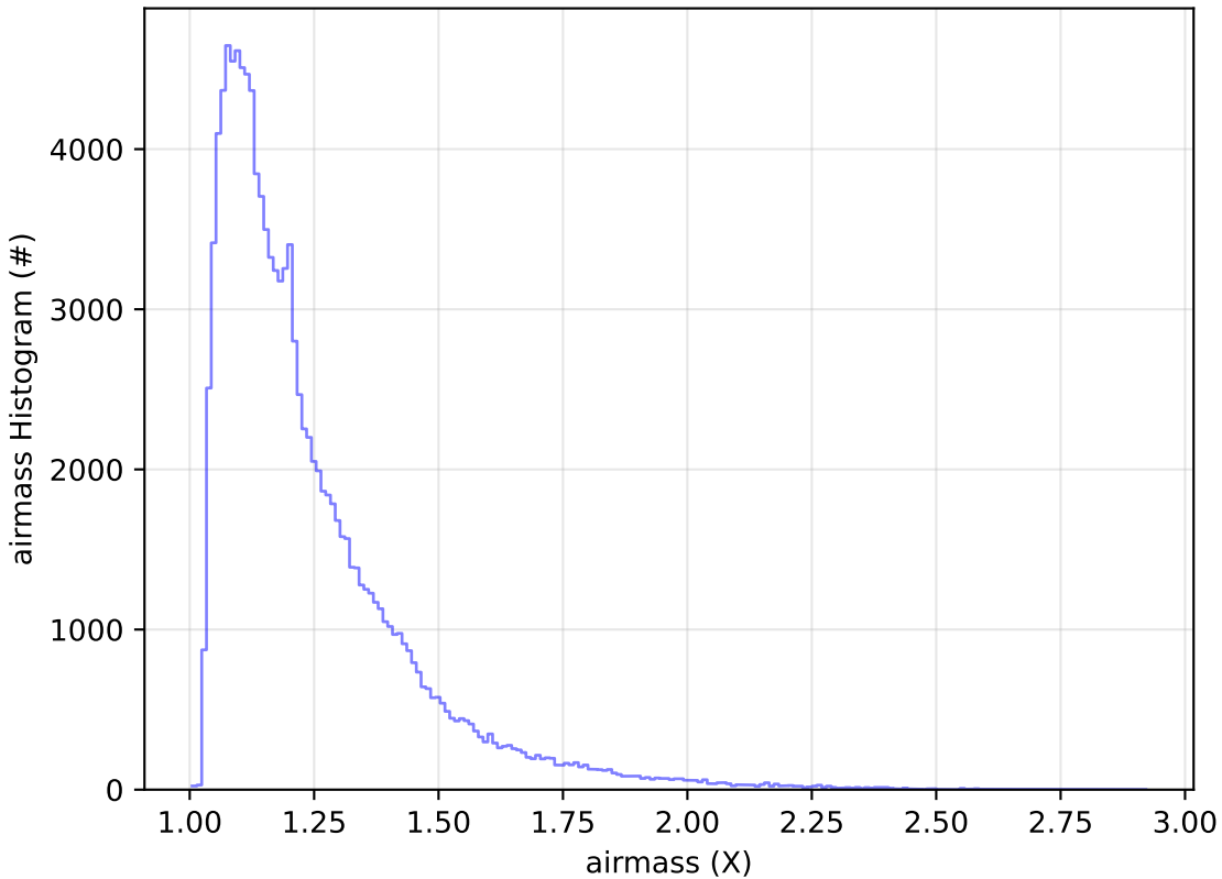
ddf_acor_sf25_lsf40_lsr10_v3.4_10yrs WFD u band: airmass Histogram
