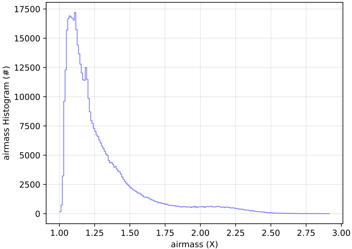
ddf_acor_sf25_Isf40_Isr10_v3.4_10yrs WFD r band: airmass Histogram
