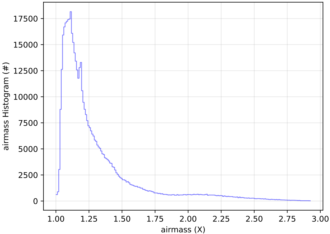
ddf_acor_sf25_lsf40_lsr10_v3.4_10yrs WFD i band: airmass Histogram
