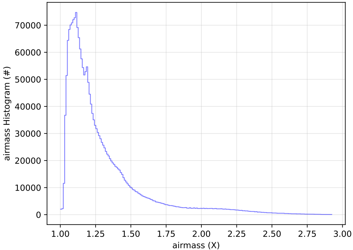
ddf_acor_sf25_lsf40_lsr10_v3.4_10yrs WFD all bands: airmass Histogram
