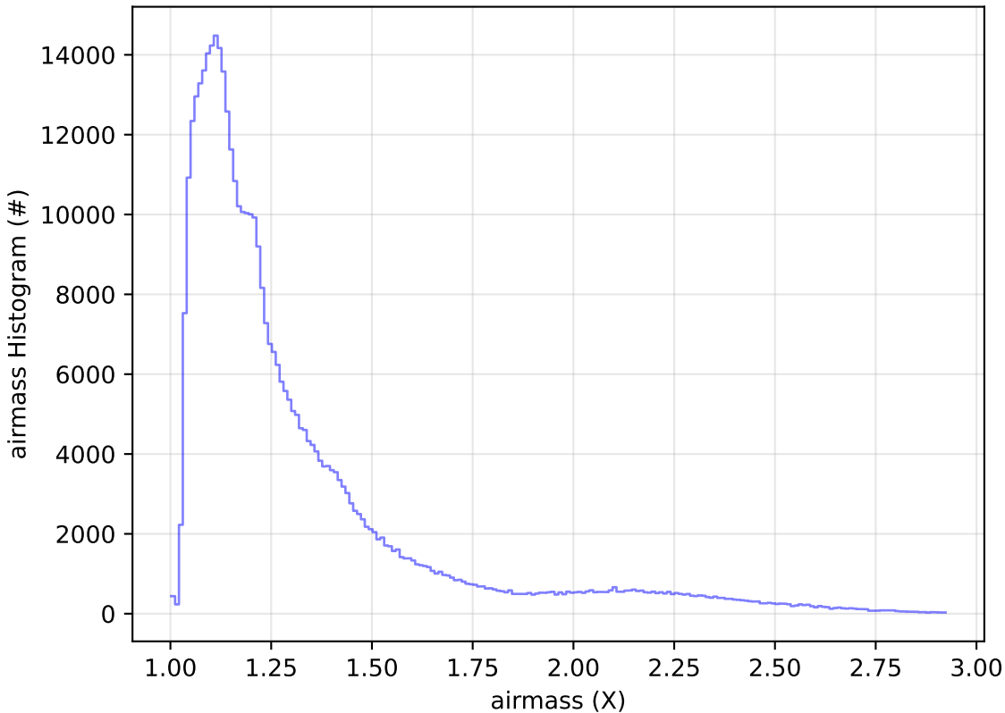
ddf_acor_sf25_lsf40_lsr10_v3.4_10yrs All sky z band: airmass Histogram
