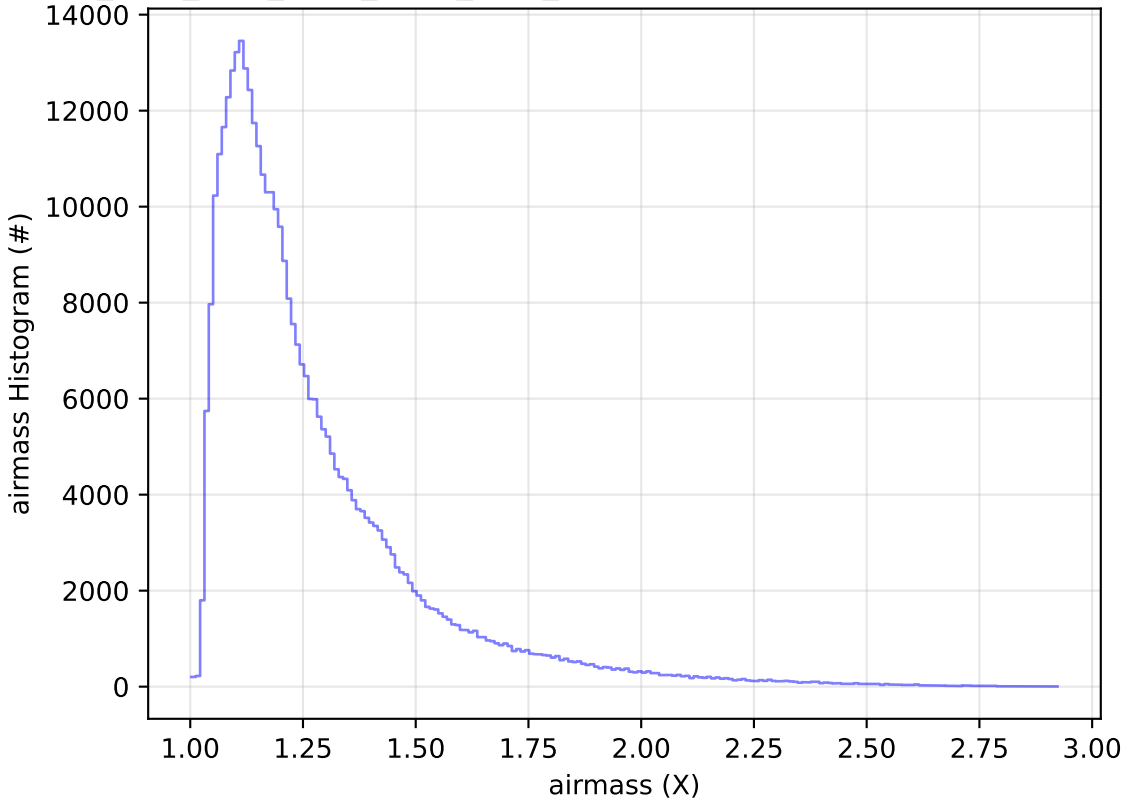
ddf_acor_sf25_ls40_lsr10_v3.4_10yrs All sky y band: airmass Histogram
