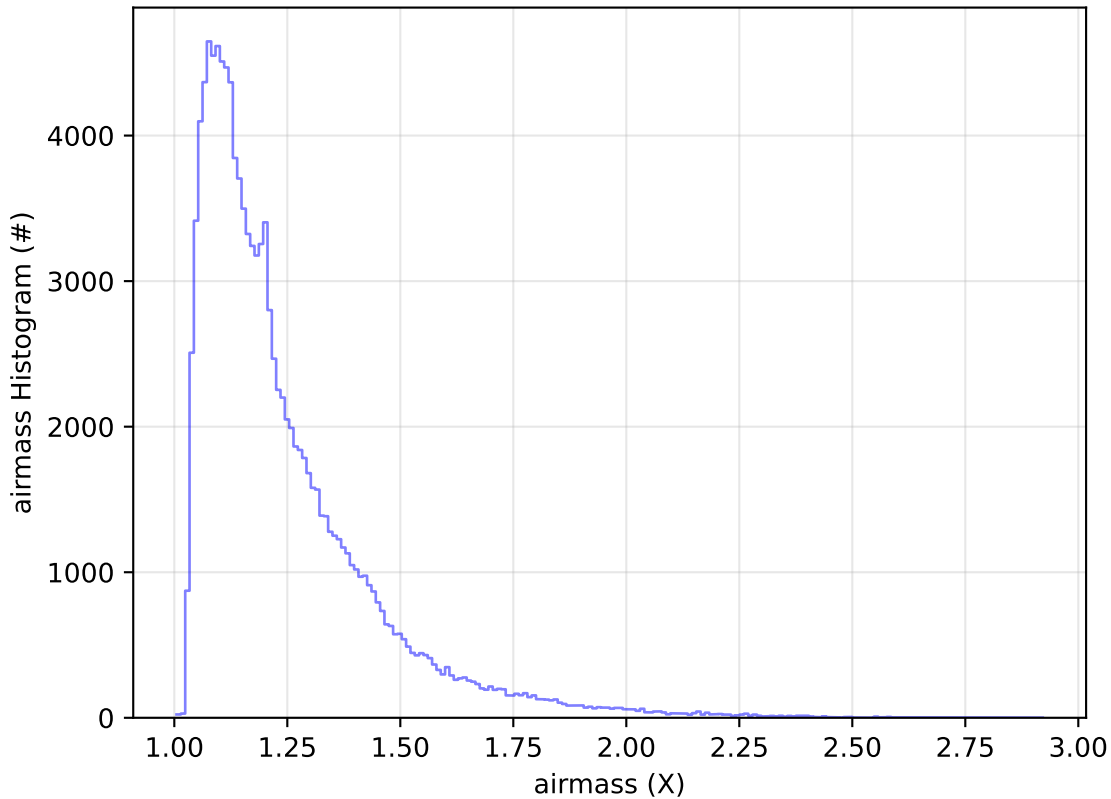
ddf_acor_sf25_lsf40_lsr10_v3.4_10yrs All sky u band: airmass Histogram
