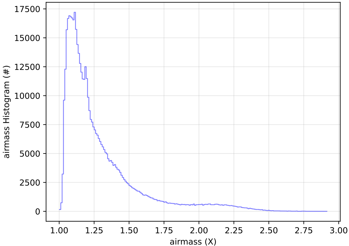
ddf_acor_sf25_lsf40_lsr10_v3.4_10yrs All sky r band: airmass Histogram
