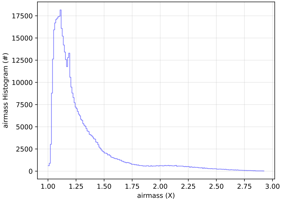
ddf_acor_sf25_lsf40_lsr10_v3.4_10yrs All sky i band: airmass Histogram
