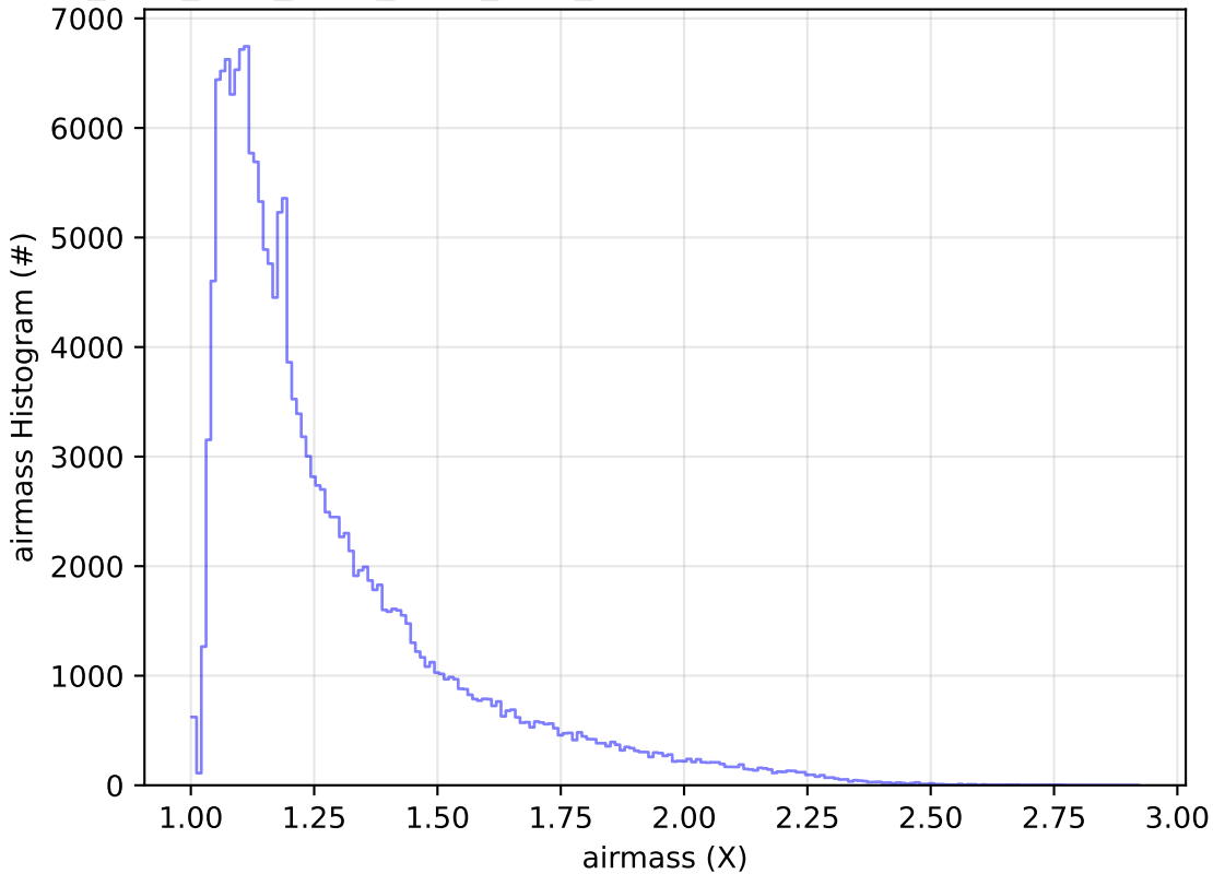
ddf_acor_sf25_lsf40_lsr10_v3.4_10yrs All sky g band: airmass Histogram
