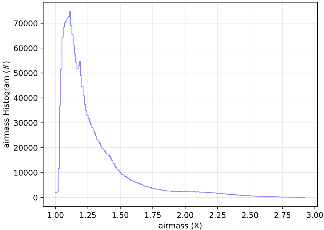
ddf_acor_sf25_lsf40_lsr10_v3.4_10yrs All sky all bands: airmass Histogram
