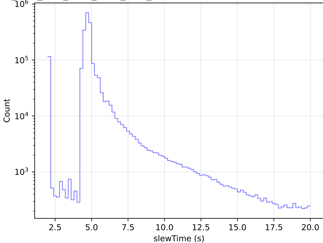
ddf_acor_sf25_Isf40_Isr10_v3.4_10yrs All visits: Zoom Slew Time Histogram
