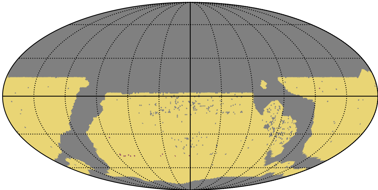
ddf_acor_sf25_lsf40_lsr10_v3.4_10yrs WFD: RapidRevisits
