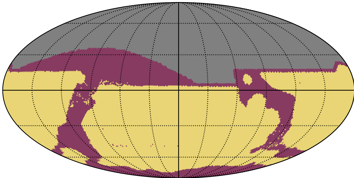
ddf_acor_sf25_lsf40_lsr10_v3.4_10yrs All sky: RapidRevisits
