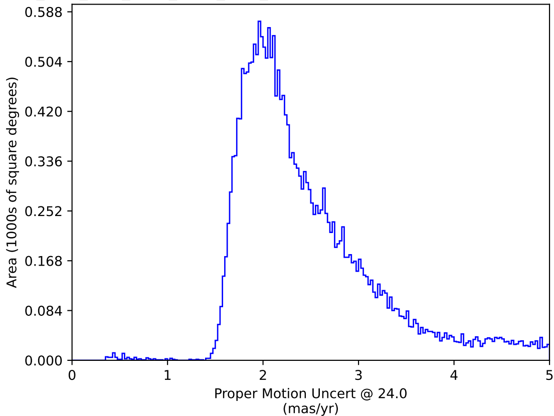
ddf_acor_sf25_lsf40_lsr10_v3.4_10yrs All sky: Proper Motion Uncert @ 24.0
