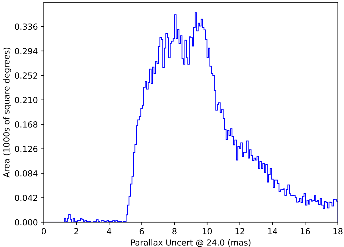
ddf_acor_sf25_lsf40_lsr10_v3.4_10yrs All sky: Parallax Uncert @ 24.0
