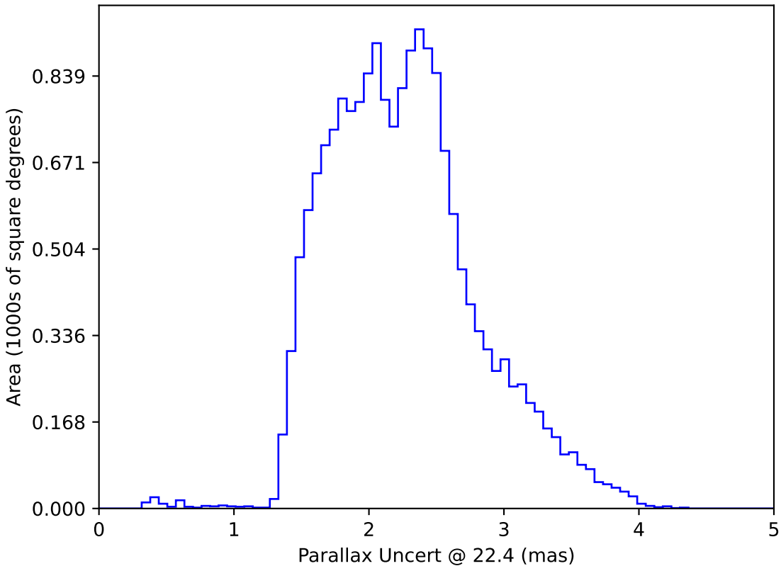
ddf_acor_sf25_lsf40_lsr10_v3.4_10yrs WFD: Parallax Uncert @ 22.4
