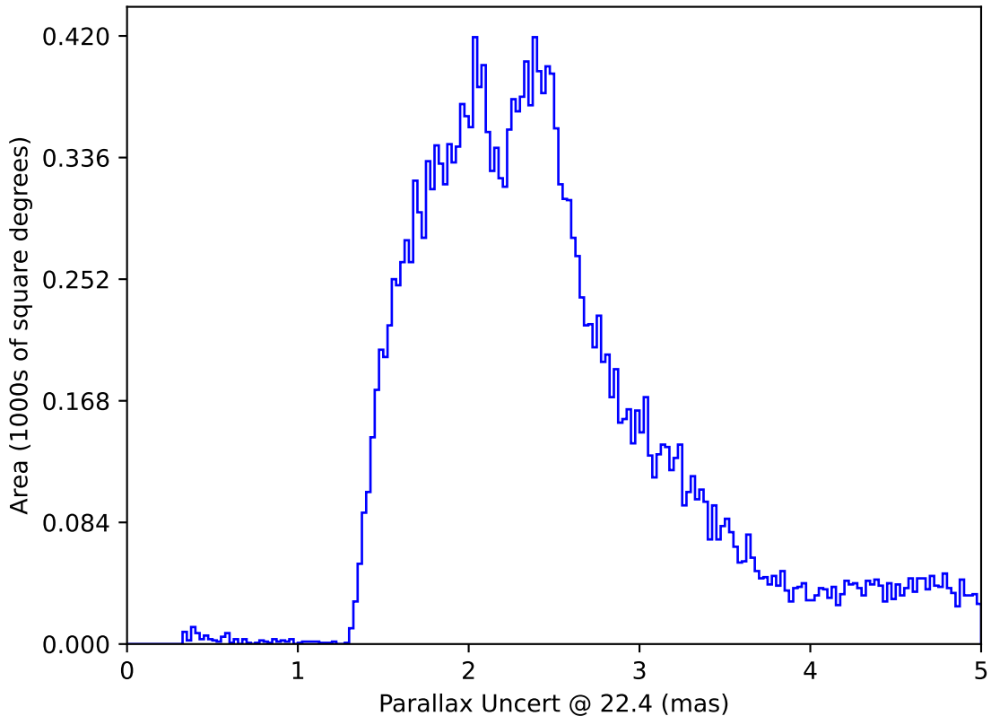
ddf_acor_sf25_lsf40_lsr10_v3.4_10yrs All sky: Parallax Uncert @ 22.4
