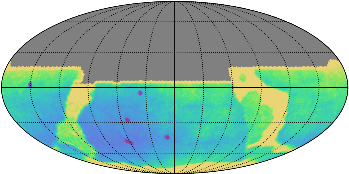
ddf_acor_sf25_lsf40_lsr10_v3.4_10yrs All sky y band only: Parallax Uncert @ 21.3
