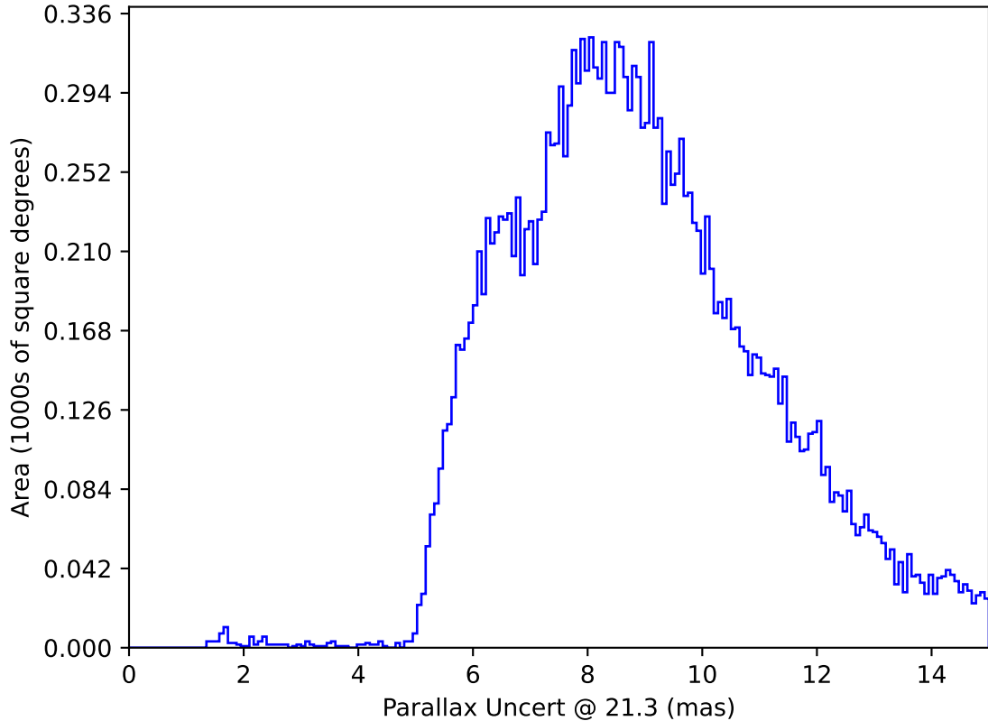
ddf_acor_sf25_lsf40_lsr10_v3.4_10yrs All sky y band only: Parallax Uncert @ 21.3
