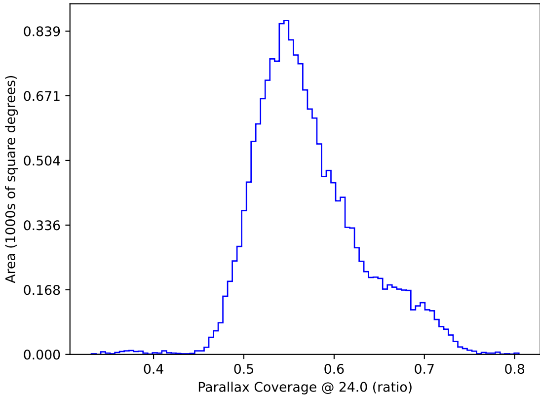
ddf_acor_sf25_lsf40_lsr10_v3.4_10yrs WFD: Parallax Coverage @ 24.0
