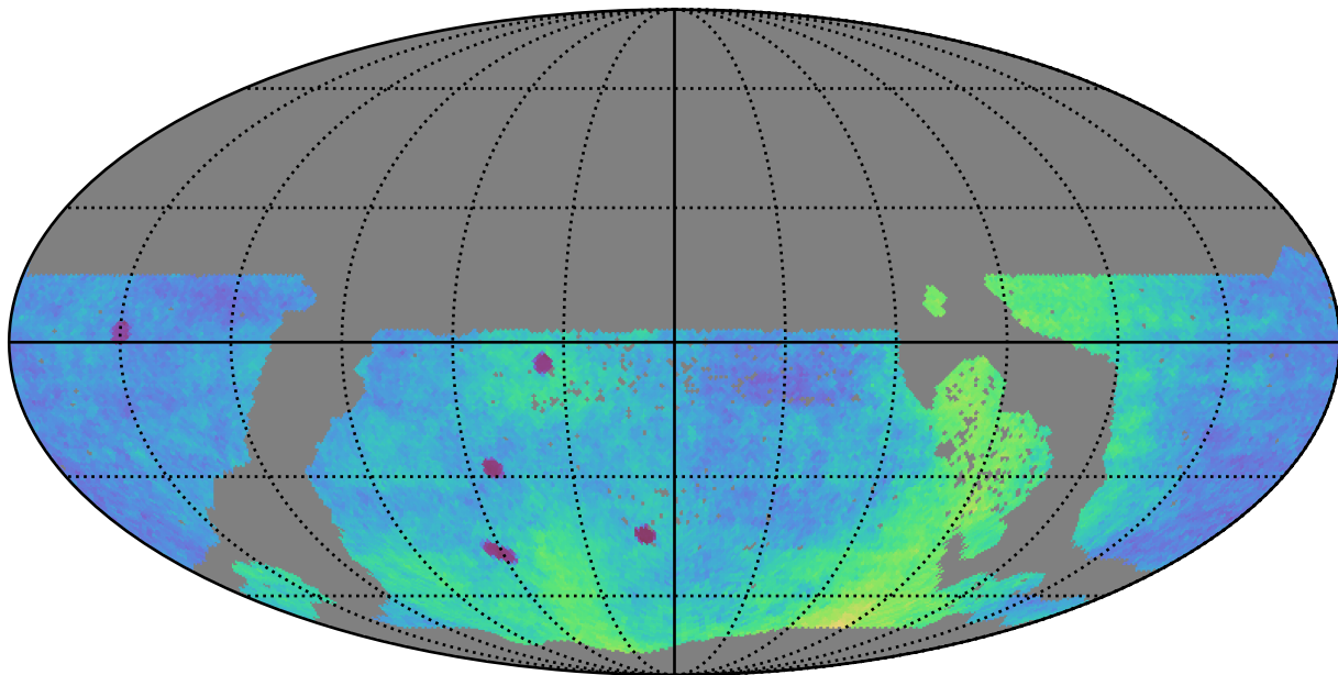
ddf_acor_sf25_lsf40_lsr10_v3.4_10yrs WFD: Parallax Coverage @ 22.4
