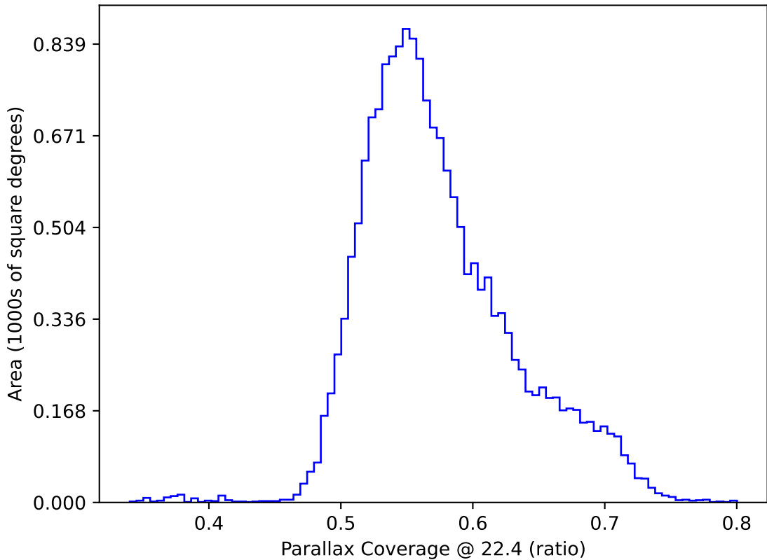
ddf_acor_sf25_lsf40_lsr10_v3.4_10yrs WFD: Parallax Coverage @ 22.4
