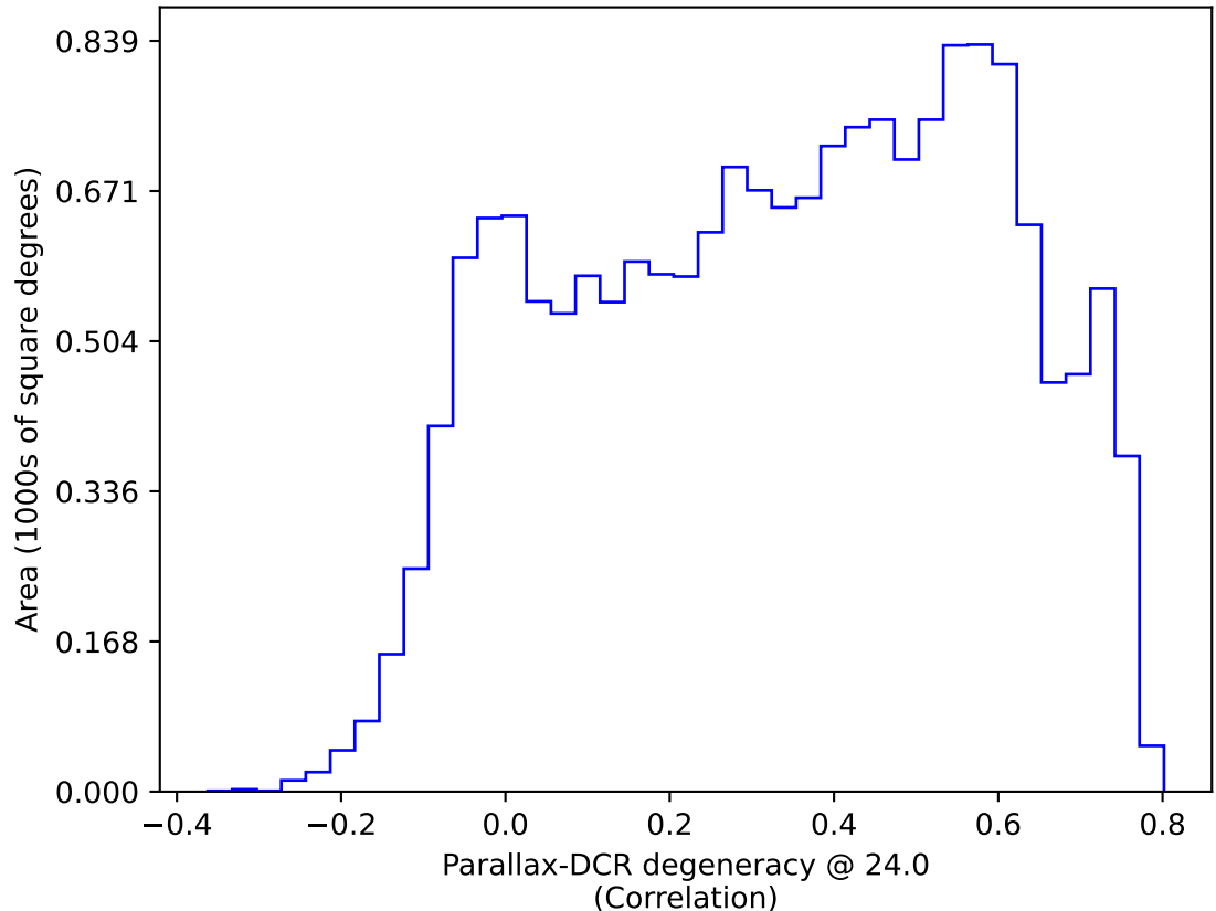
ddf_acor_sf25_lsf40_lsr10_v3.4_10yrs WFD: Parallax-DCR degeneracy @ 24.0
