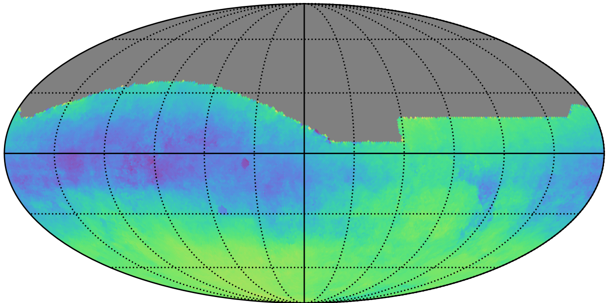
ddf_acor_sf25_lsf40_lsr10_v3.4_10yrs All sky: Parallax-DCR degeneracy @ 24.0
