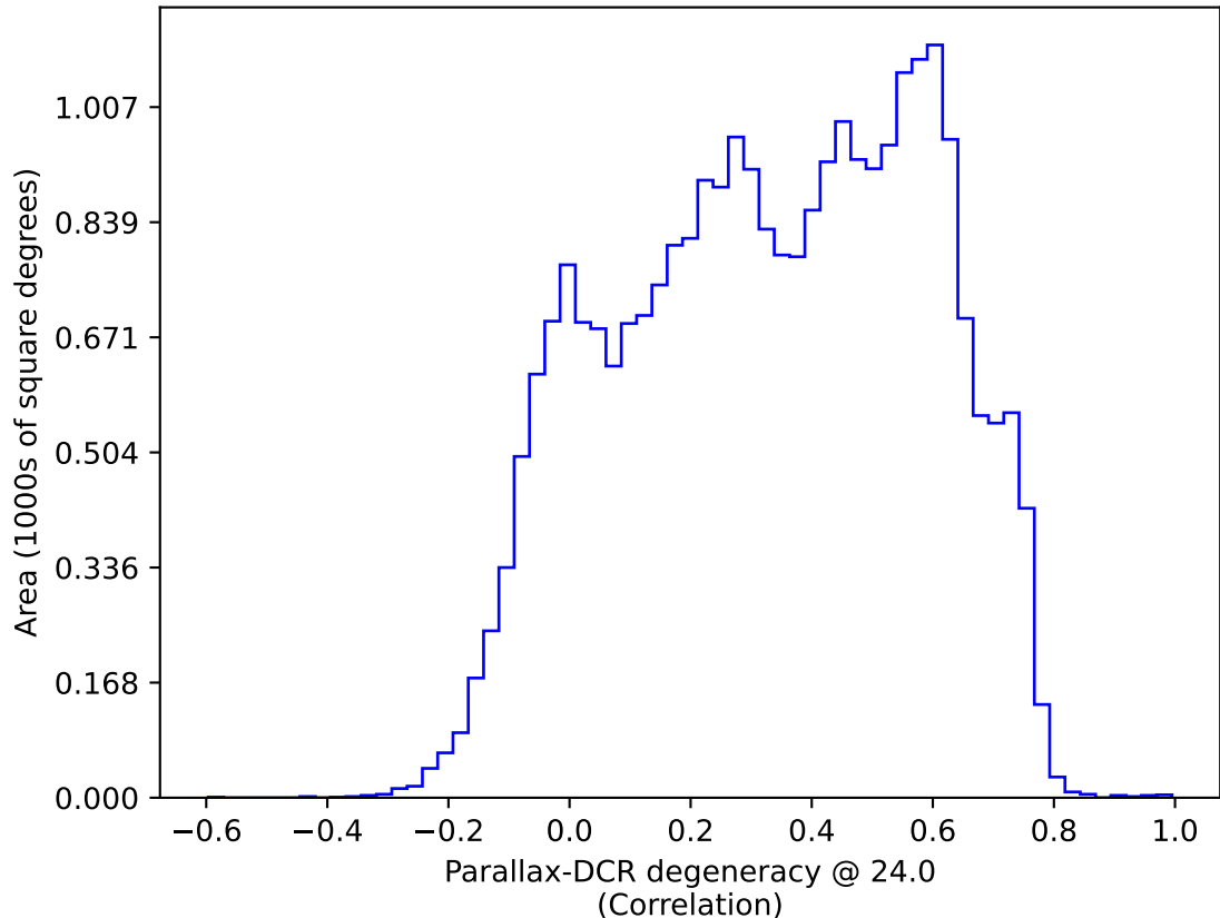
ddf_acor_sf25_lsf40_lsr10_v3.4_10yrs All sky: Parallax-DCR degeneracy @ 24.0
