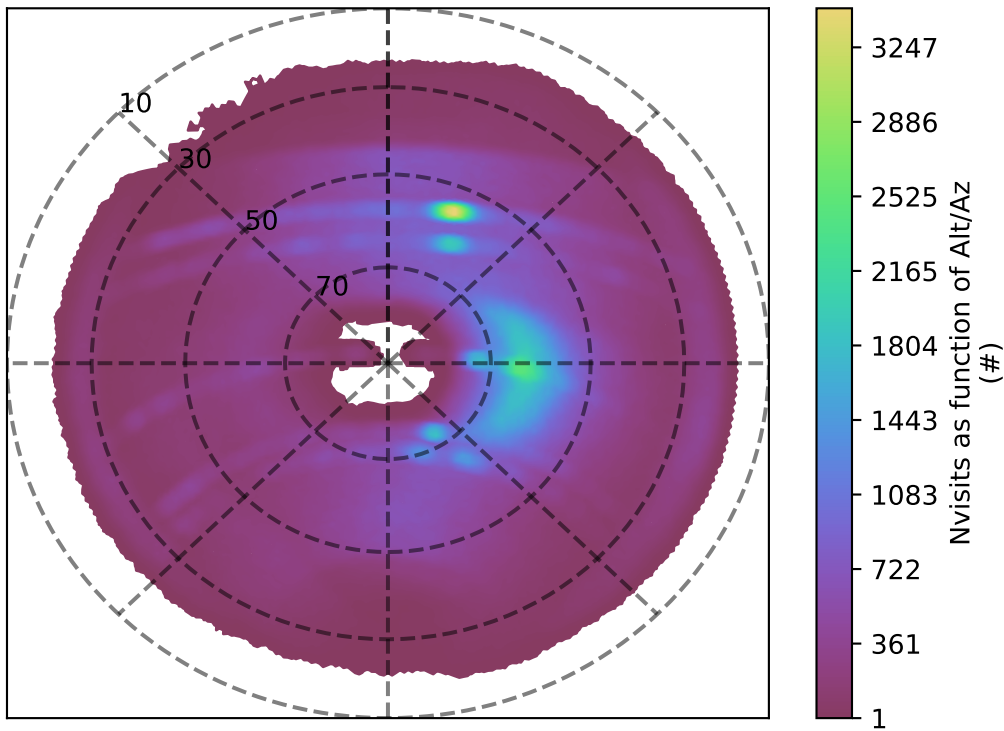
ddf_acor_sf25_lsf40_lsr10_v3.4_10yrs z band: Nvisits as function of Alt/Az
