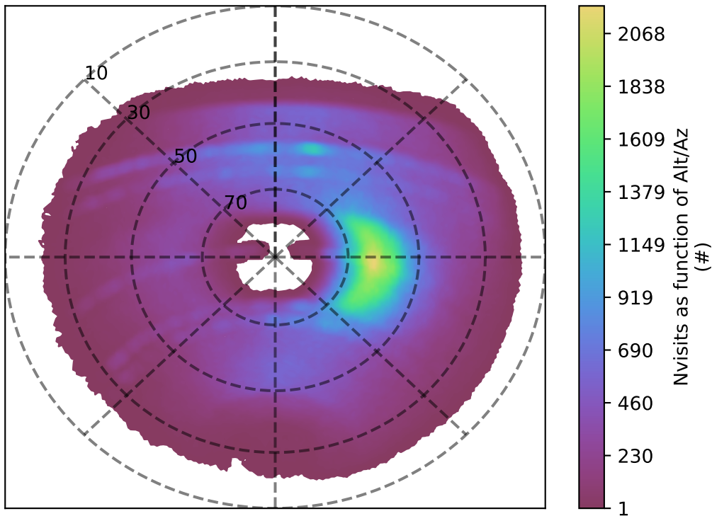
ddf_acor_sf25_lsf40_lsr10_v3.4_10yrs y band: Nvisits as function of Alt/Az
