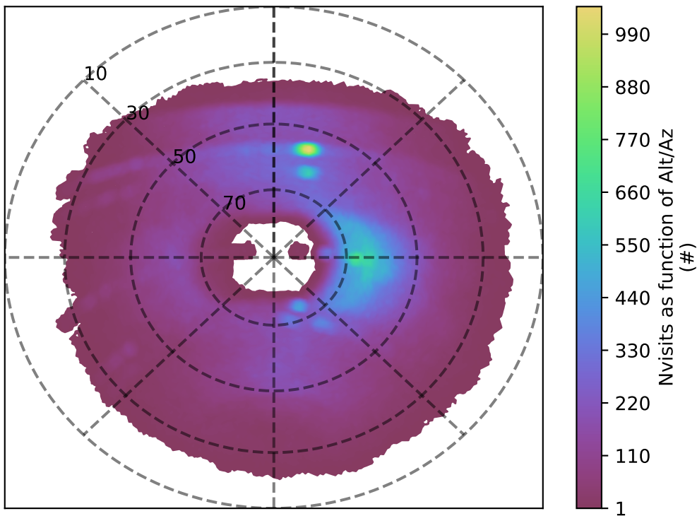
ddf_acor_sf25_lsf40_lsr10_v3.4_10yrs u band: Nvisits as function of Alt/Az
