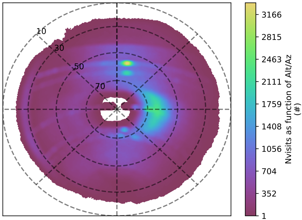
ddf_acor_sf25_lsf40_lsr10_v3.4_10yrs r band: Nvisits as function of Alt/Az
