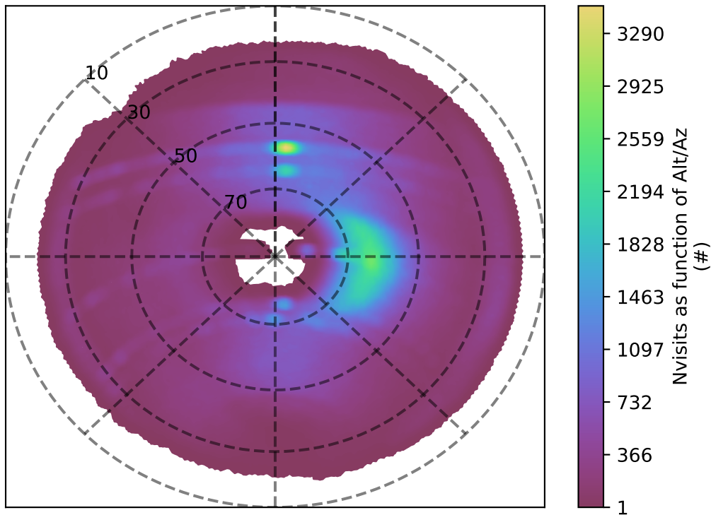
ddf_acor_sf25_lsf40_lsr10_v3.4_10yrs i band: Nvisits as function of Alt/Az
