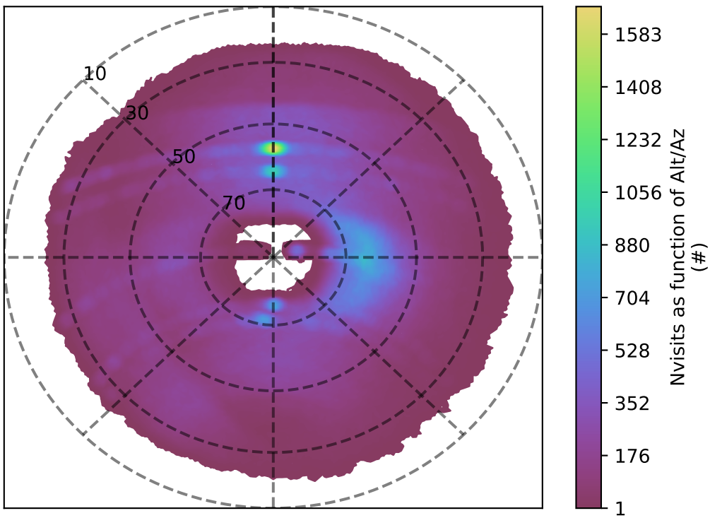
ddf_acor_sf25_lsf40_lsr10_v3.4_10yrs g band: Nvisits as function of Alt/Az
