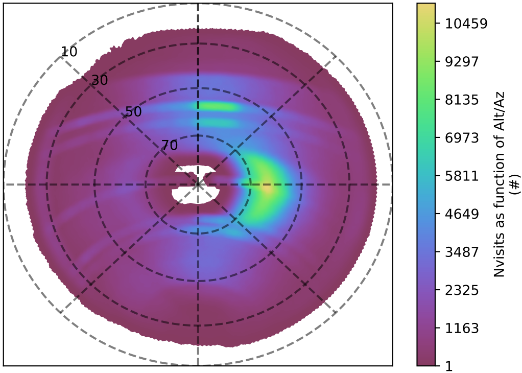
ddf_acor_sf25_ls40_lsr10_v3.4_10yrs all bands: Nvisits as function of Alt/Az
