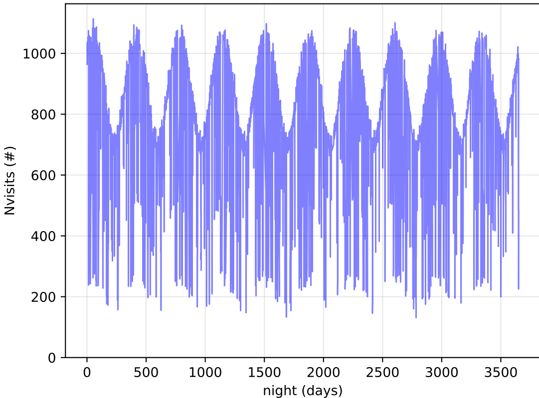
ddf_acor_sf25_lsf40_lsr10_v3.4_10yrs All visits: Nvisits
