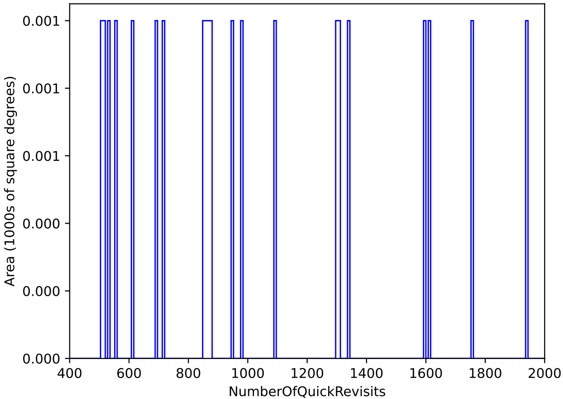
ddf_acor_sf25_lsf40_lsr10_v3.4_10yrs WFD: NumberOfQuickRevisits
